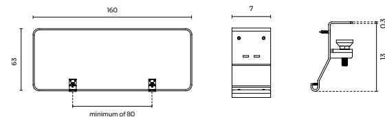
Measurements AK 3 Desk Clamp
