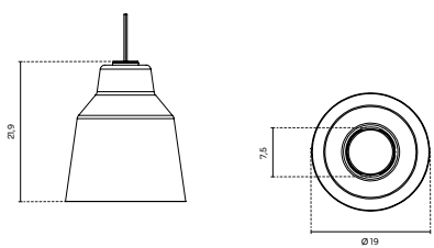
Measurements Ratio 29 Pendant Lamp
