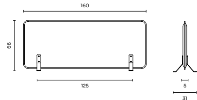
Measurements AK 3 Desk Clamp
